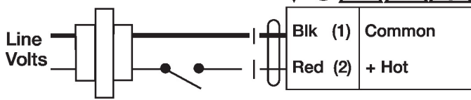
24 VAC Transformer
