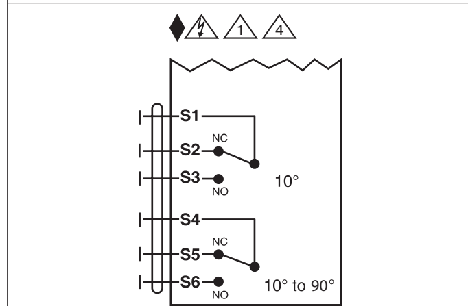
Auxiliary Switches
