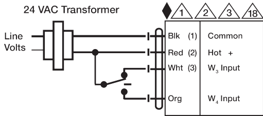
Floating Point
