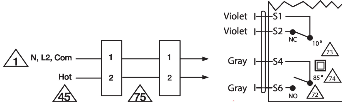
Parallel Actuator Wiring
