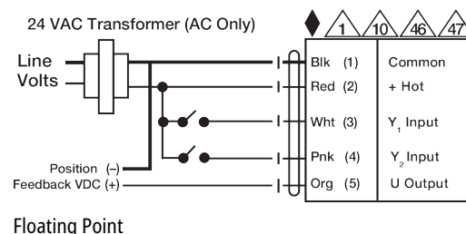
Floating Point
