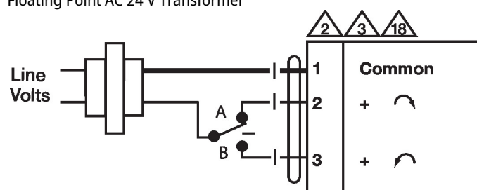
Floating Point AC 24 V Transformer
