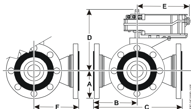
Figure 5: M9220 Actuated VG18A5xx Three-Way Series Ball Valves
