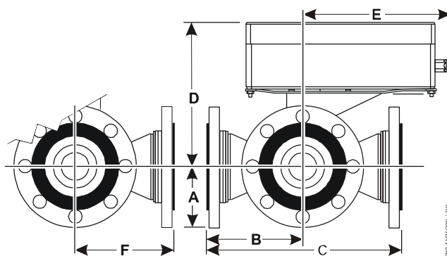
Figure 9: Actuated VG18A5xx Three-Way Series Ball Valves with M9000-340 Weathershield
