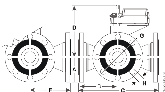
Figure 3: M9124 Actuated VG18A5xx Three-Way Series Ball Valves
