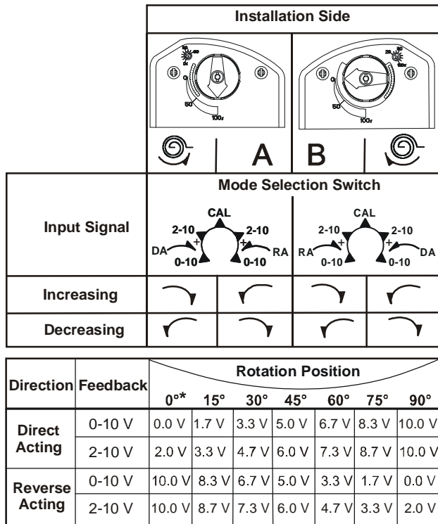
Figure 24: Control Response
