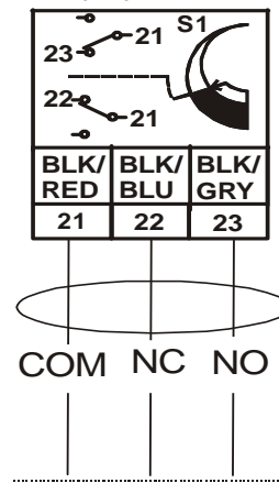
Figure 21: Auxiliary Switch Wiring Diagram
