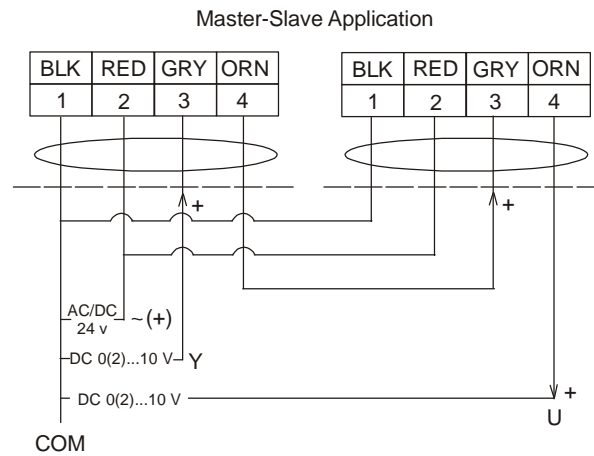
Figure 19: Control Wiring Diagrams
