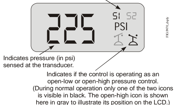
Figure 3: P470 Control Operating Display
