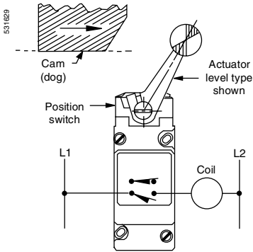
Figure 3 - Limit switch
