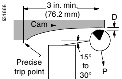
Fig "1c" cam design for speeds between 200 fpm and 400 fpm (60.9 mpm and 121.9 mpm).
