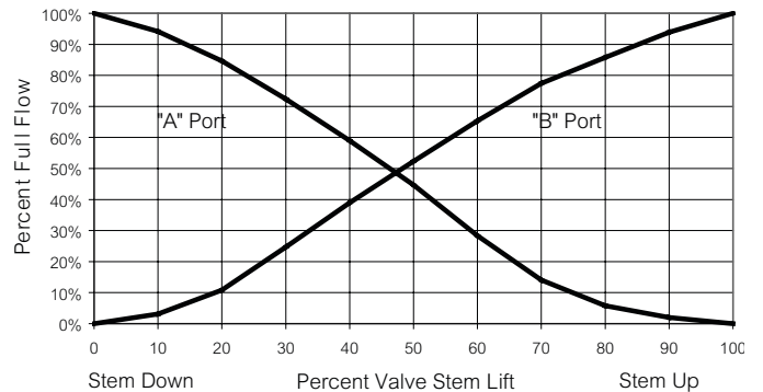
Figure-25 Typical Flow Characteristics
