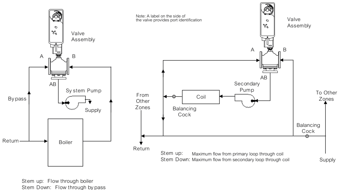
Figure-28 Typical Piping Choices for VB-8303 as 3-Way Mixing Valve for Proportional Control Used to Blend Two Water Flows.
