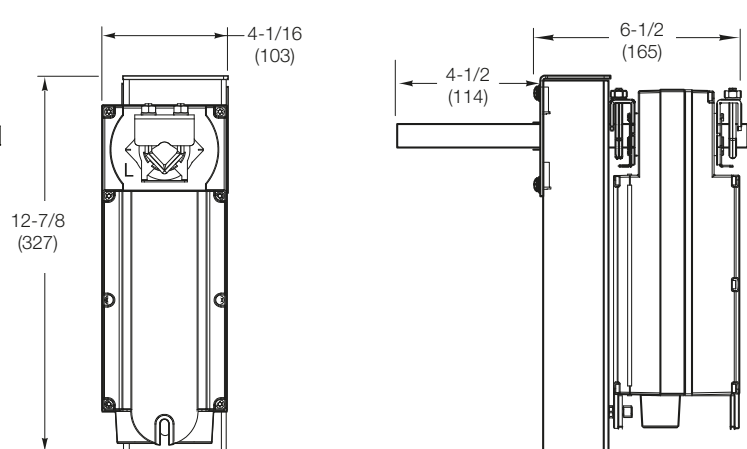
Figure 15 Mx40-717x-230 Actuator/Linkage Assembly
