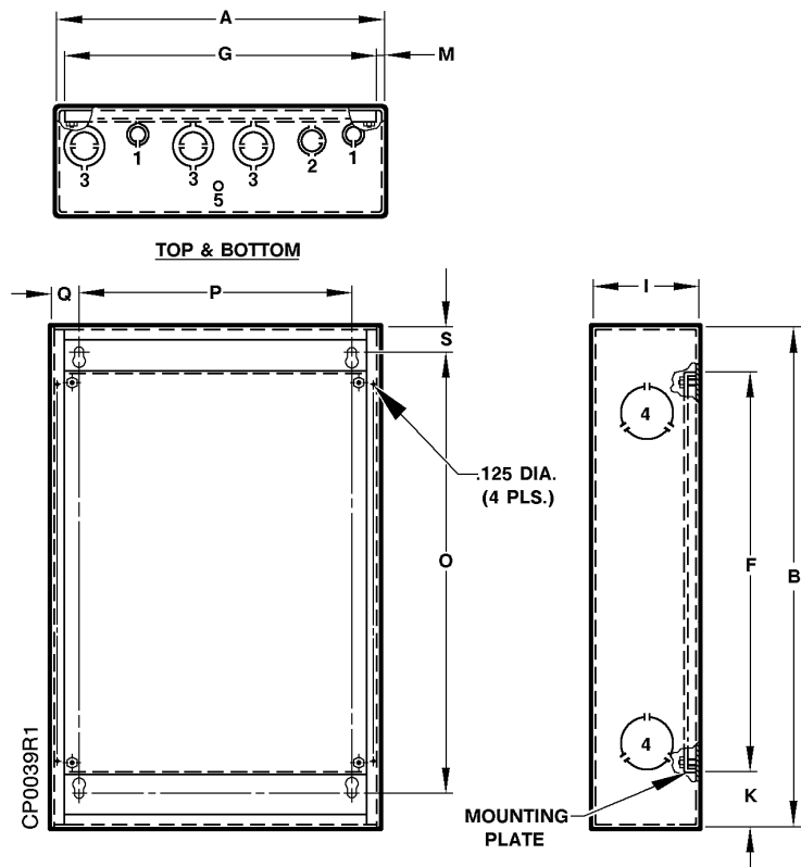
Figure 6. Flush Mount Cabinet Dimensions (See Table 7).
