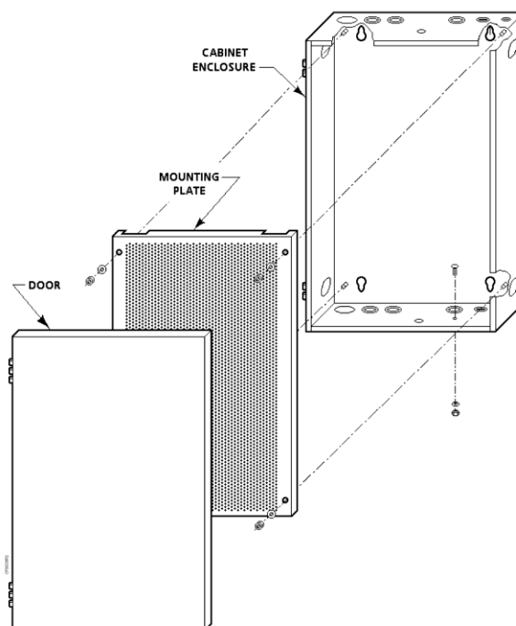
Figure 2. Wall Mount Cabinet Components.
