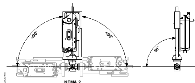
Figure 11. Acceptable NEMA 2 Mounting Positions. Wiring.
