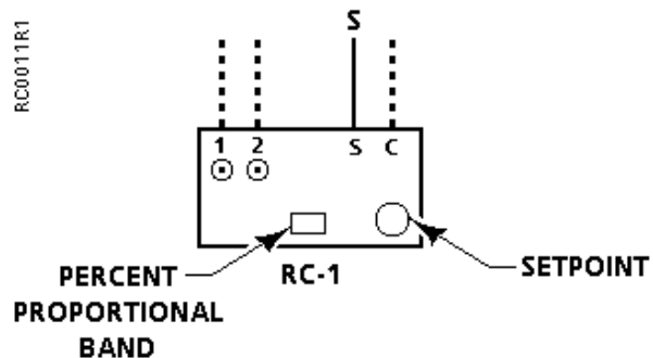
Figure 3. Calibration Settings.
