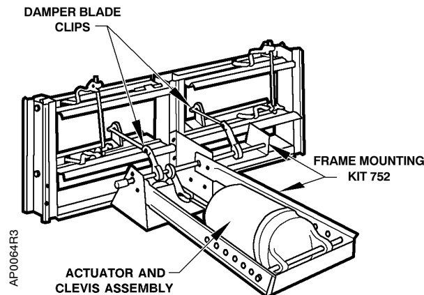
Figure 5. Two-section Damper.
