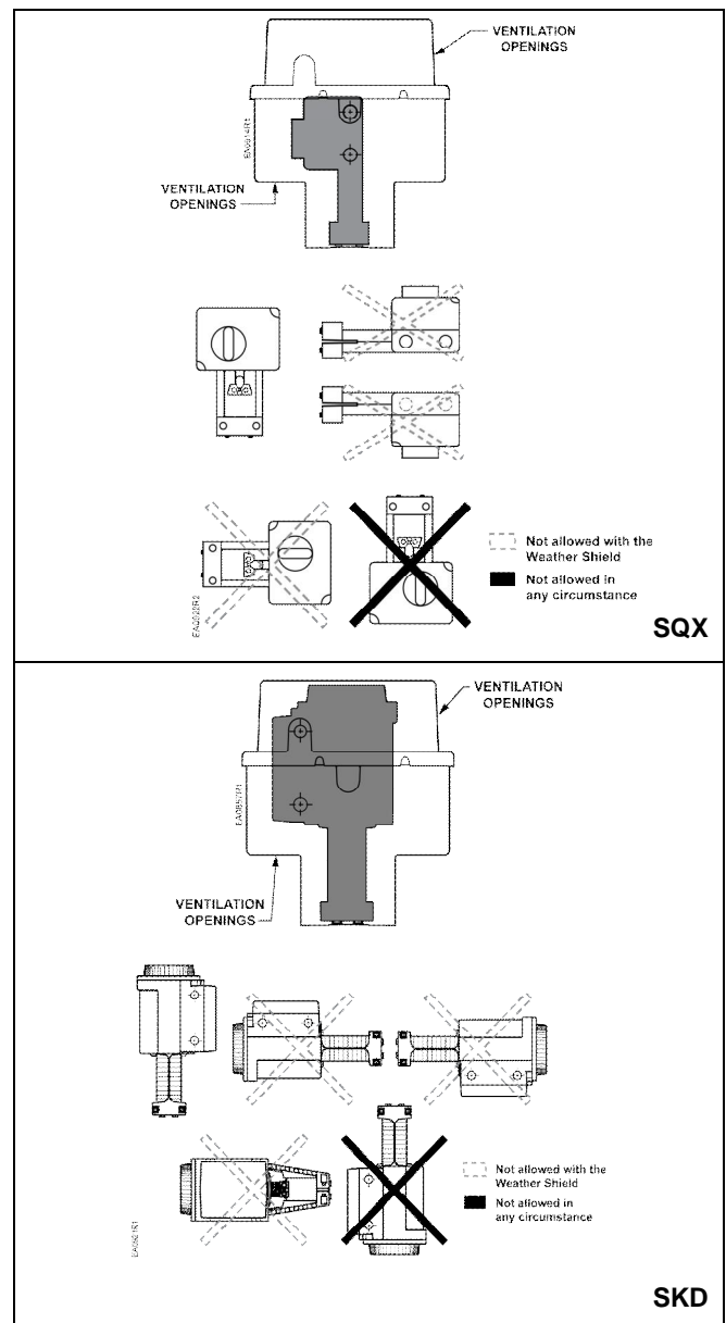
Figure 1. Mounting Orientation.
